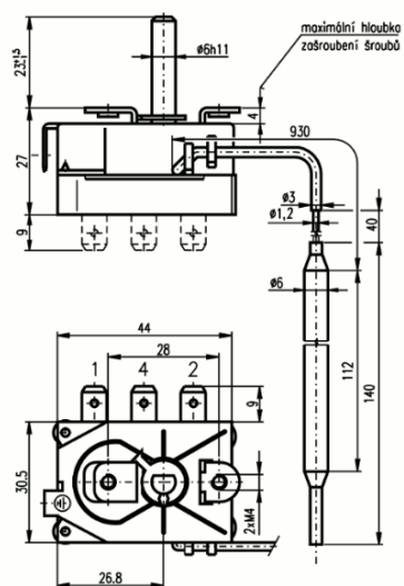
Wiring scheme in open position
