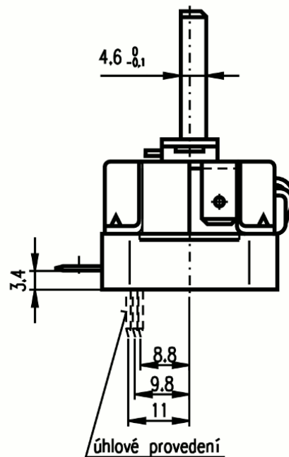
Wiring scheme in open position
